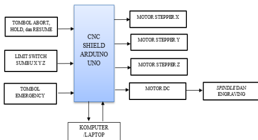
Gambar 6 Gambar Diagram Blok
