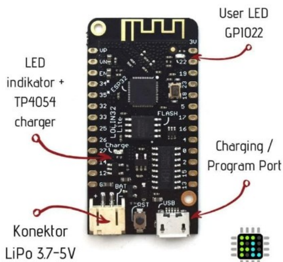
Figure 2.11. ESP 32 to read and trasmit data
