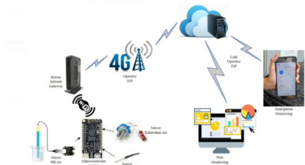
Figure 2.7. Research IoT Network Infrastructure To measure the pH of pool water, a pH sensor is used which is capable of measuring pH from 0 to 18, shown in figure 2.8
