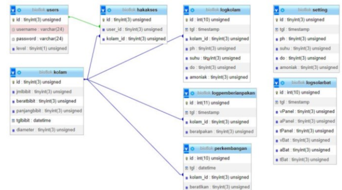
Figure 2.3. Relationships between tables in a MySQL database
