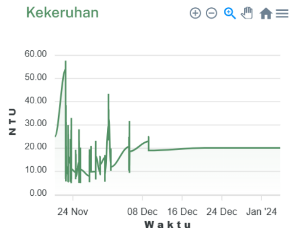
Figure 3.7. Turbidity grafic
