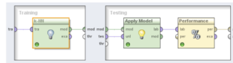
Figure 4. KNN Testing
