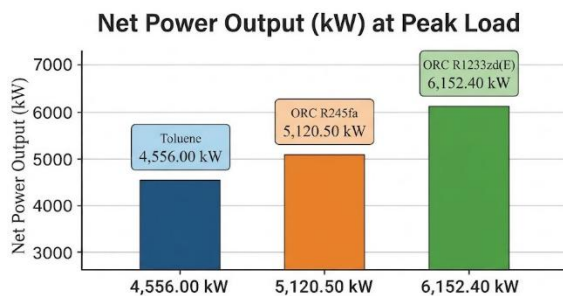
Figure 1. Peak Net Power Generation across Candidate Fluids
