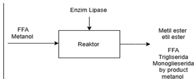
Fig. 8. Proposed reaction mechanism of enzymatic esterification catalyzed by free lipase enzyme from oil palm mesocarp
