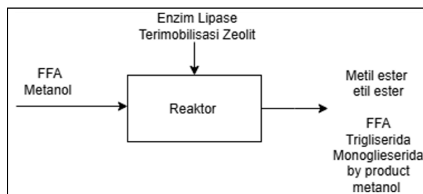
Fig. 9. Proposed reaction mechanism of enzymatic esterification catalyzed by zeolite-immobilized lipase enzyme
