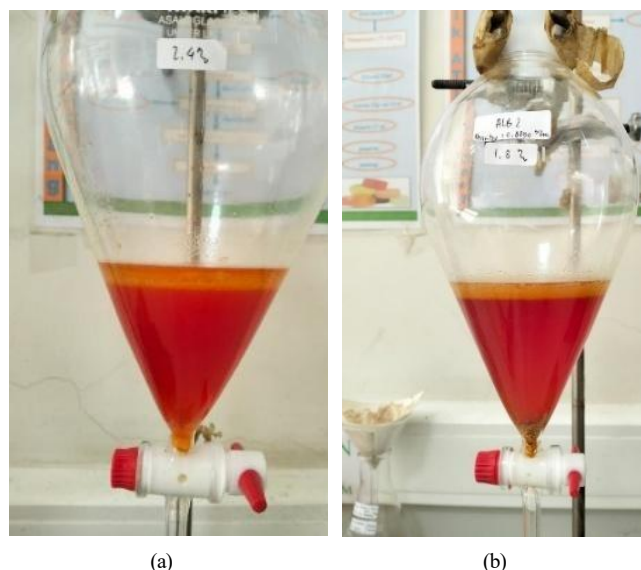
Fig. 7. Biodiesel products obtained using (a) free lipase from oil palm mesocarp and (b) zeolite-immobilized lipase
