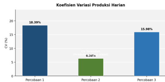
Fig. 3. Graph of the Coefficient of Variation (CV) of Daily Biogas Production per Trial
