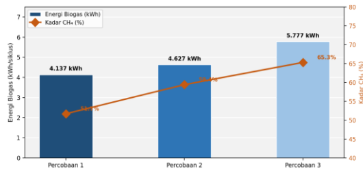
Fig. 4. Graph of the Relationship between CH 4 Content and Biogas Energy per Cycle
