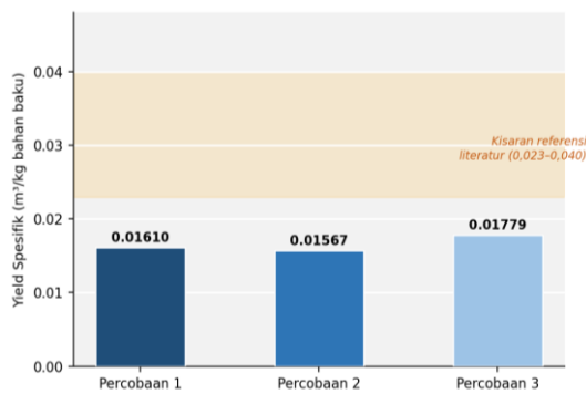
Fig. 1. Graph of the Specific Yield per Trial
