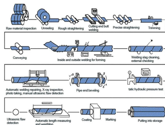
Fig. 1. SAW Pipe Manufacturing Process [1]
