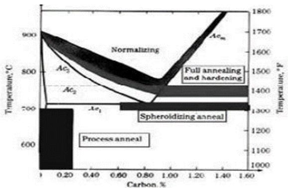
Fig. 3. Diagram of Temperature Relationship with Heat Treatment on carbon steel [5]
