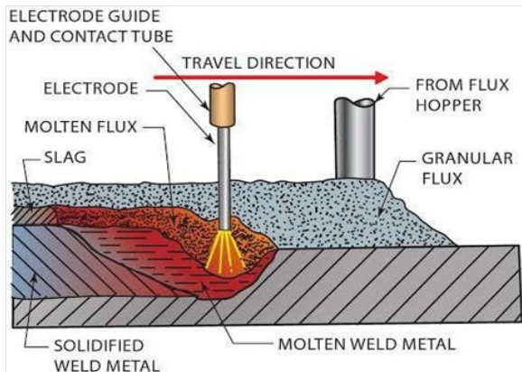
Fig. 2. SAW Welding Process
