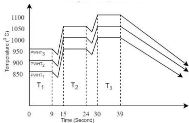
Fig. 6. PWHT Temperature Diagram
