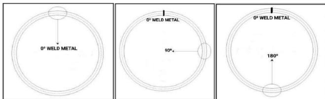
Fig. 5. Cutting Pipe Specimens Residual Stress Testing
