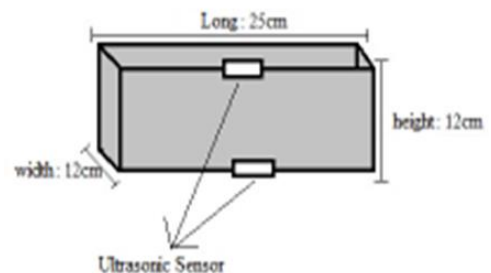
Fig. 4. Gondola cage prototype design
