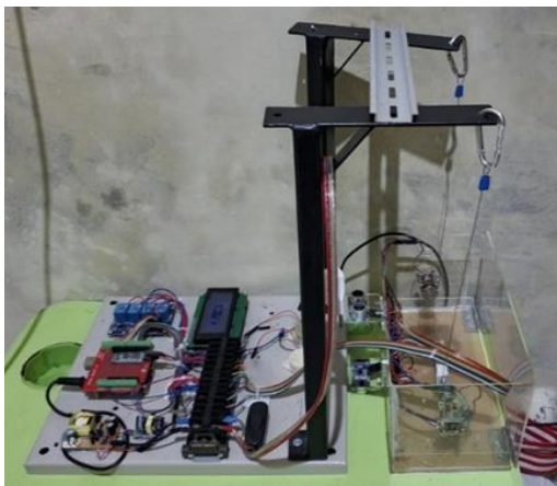
Fig. 6. Prototype system
