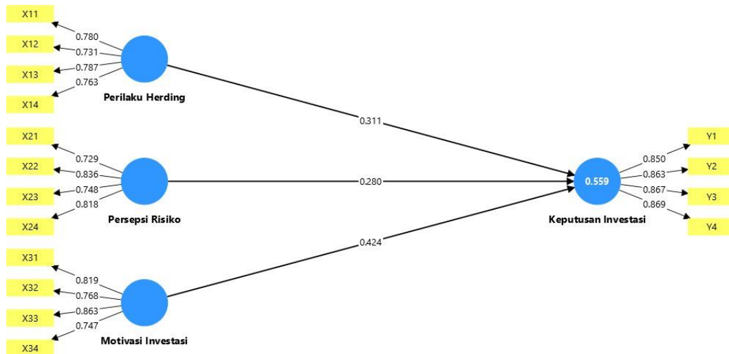
Figure 2 Measurement Model (Outer Model)
